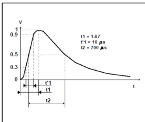
Fig. 1 CCITT 7 10/700 μs surge definition
