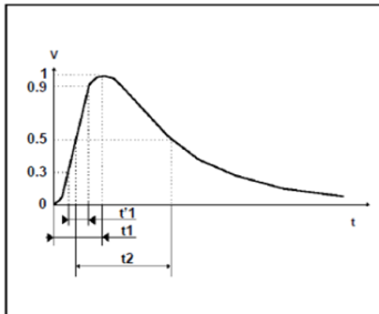
Fig. 1 8/20 µs surge definition
